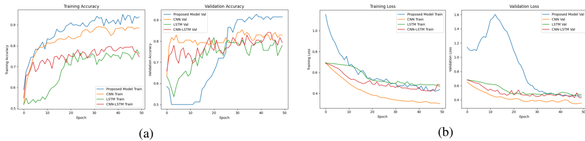
Figure 2. Training and validation performance curves for dataset 1: (a) accuracy curves and (b) loss curves
