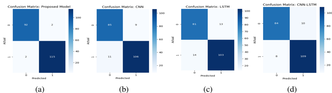
Figure 6. Confusion matrix for dataset 2: (a) proposed model, (b) CNN, (c) LSTM, and (d) CNN-LSTM
