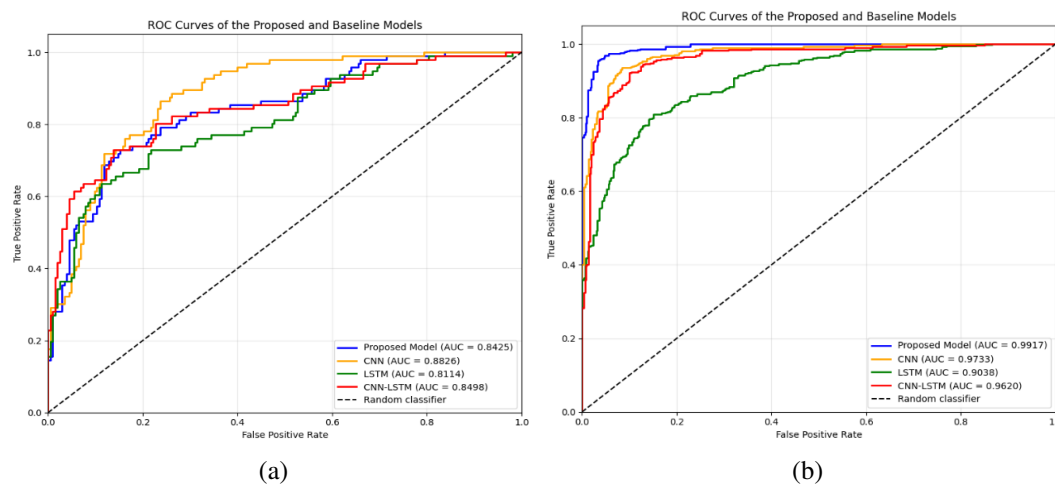
Figure 7. ROC curve: (a) dataset 1 and (b) dataset 2
