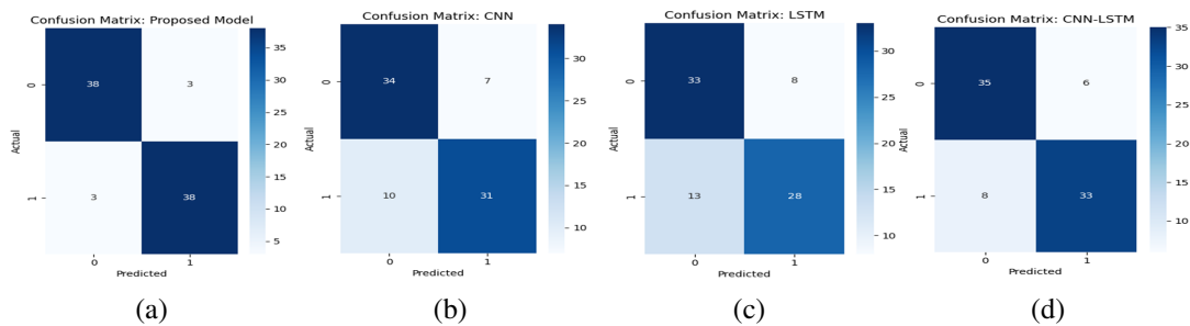
Figure 5. Confusion matrix for dataset 1: (a) proposed model, (b) CNN, (c) LSTM, and (d) CNN-LSTM
