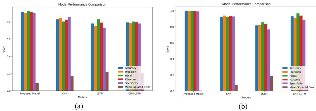
Figure 4. Comparison graphs: (a) dataset 1 and (b) dataset 2
