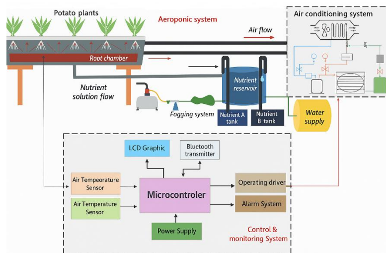
Figure 2. Aeroponic system architecture
