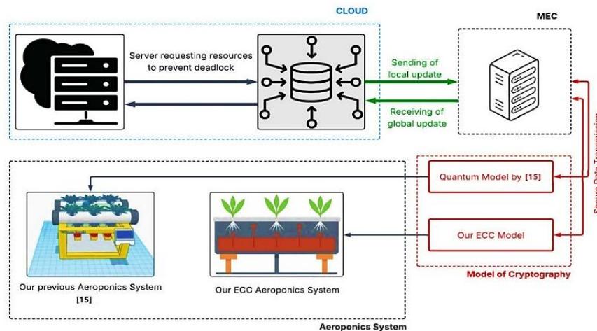
Figure 1. FL architecture integrating the previous BB84-based system and the proposed ECC-based system through a central aggregation server
