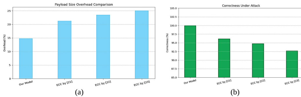
Figure 4. Performance benchmark; (a) payload size overhead and (b) correctness under targeted attacks
