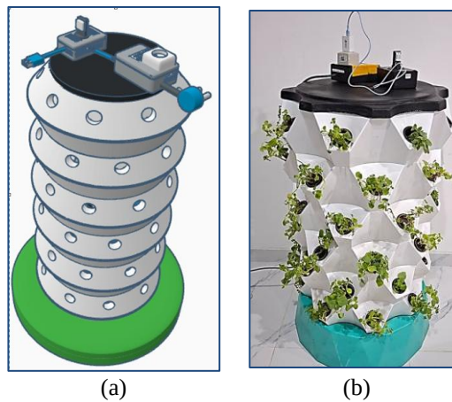
Figure 6. System visualization; (a) conceptual structure of aeroponics cultivation module and (b) practical implementation and system integration scenario
