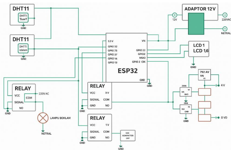
Figure 3. Aeroponic hardware design
